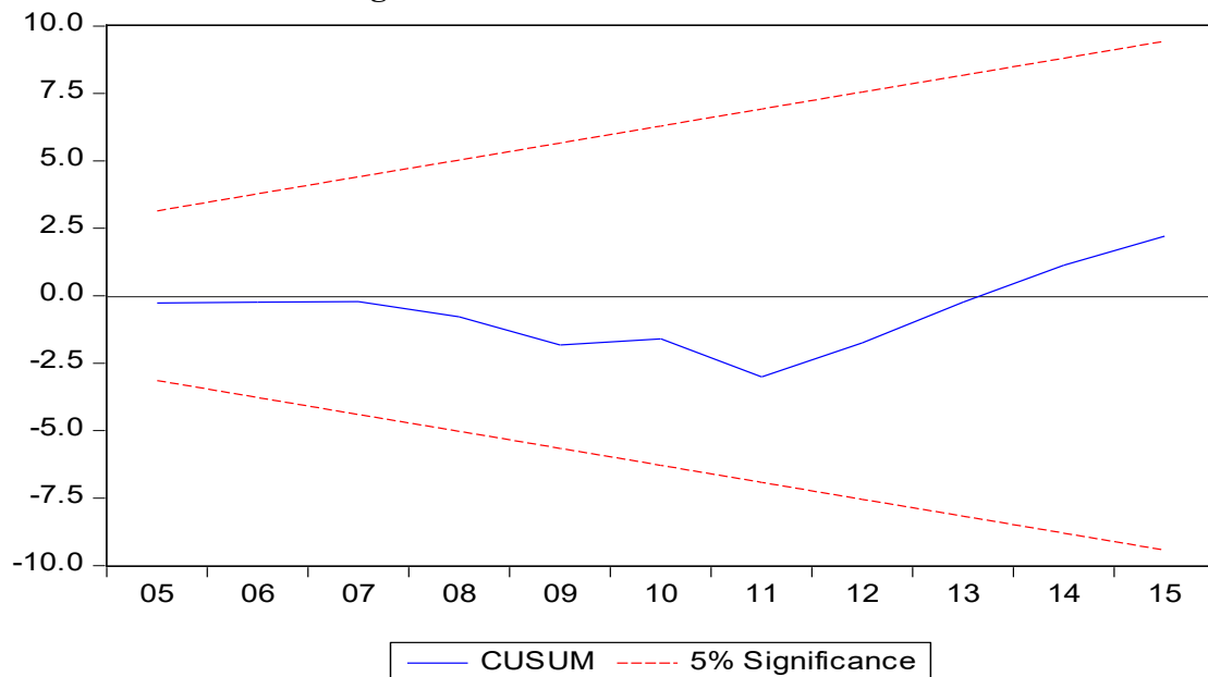
Figure 2: Plot of CUSUM for LnIMPD
